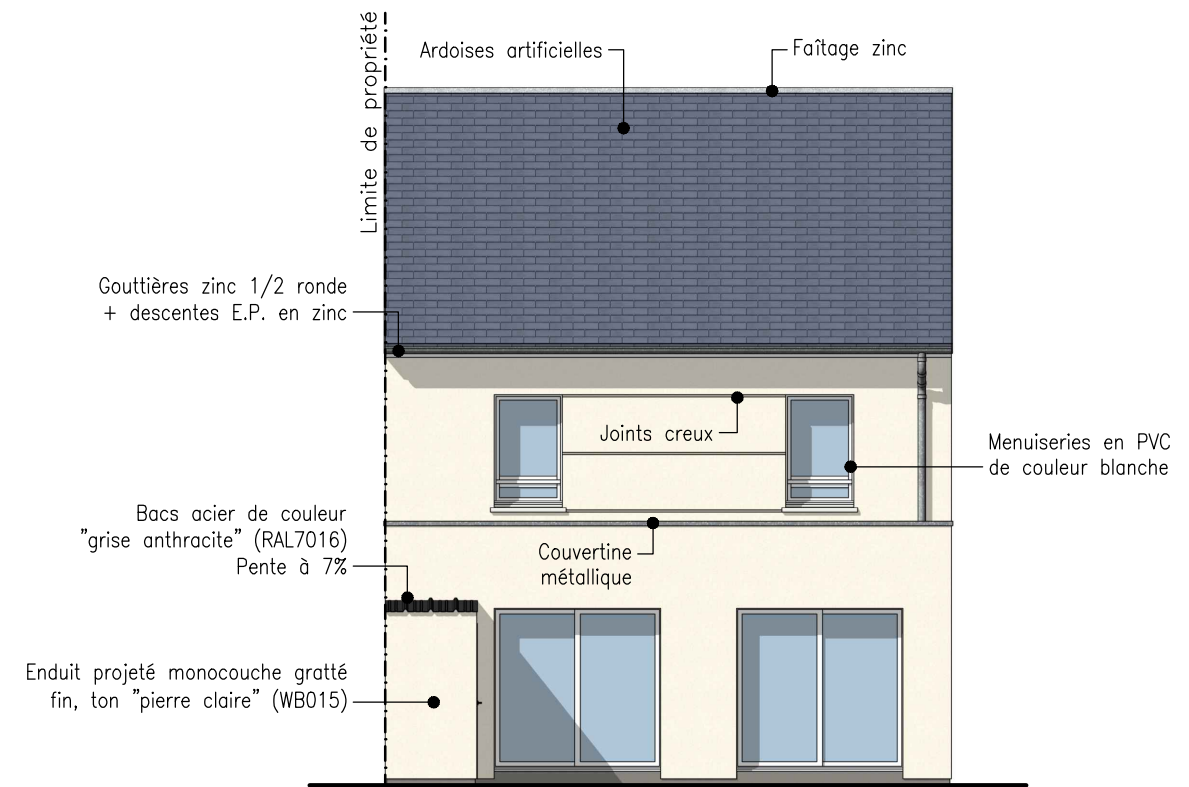
FACADE SUD
